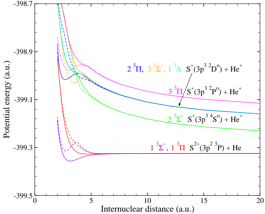
FIG. 1: (Color) The adiabatic (—) and diagonal diabatic (----) potential energies for the SHe^{2+} system as a function of internuclear distance R .
