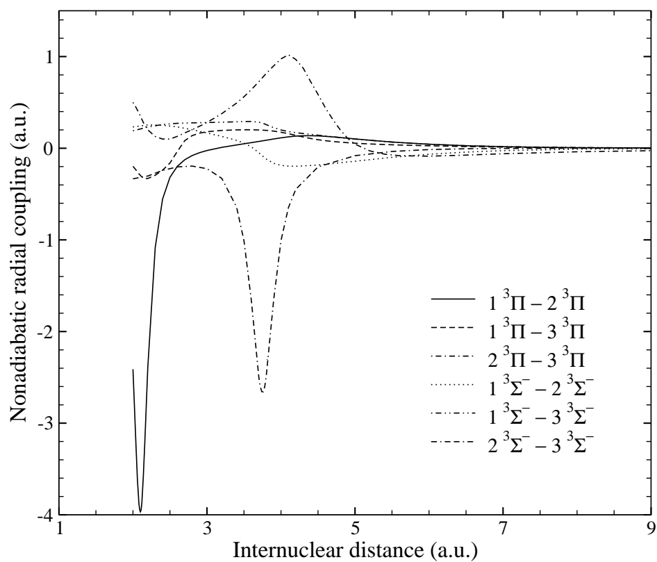
FIG. 2: The nonadiabatic radial couplings for the S\text{He}^{2+} system as a function of internuclear distance R .
