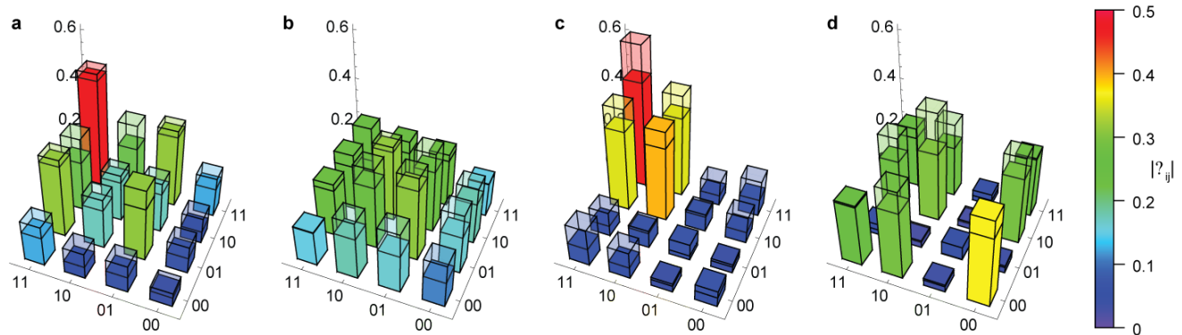
FIG. 2: Diversity of states. Examples of the density matrices created by applying four of the randomly chosen unitary transformations to simple product states. The bar heights and colors show the absolute value of the output density matrices, with the experimental data shown solid and the theory shown semi-transparent. These states have fidelities f = 0.81, 0.80, 0.75, 0.80 , relative to the ideal states. The Supplementary Information gives the input states and operations used in these examples.
