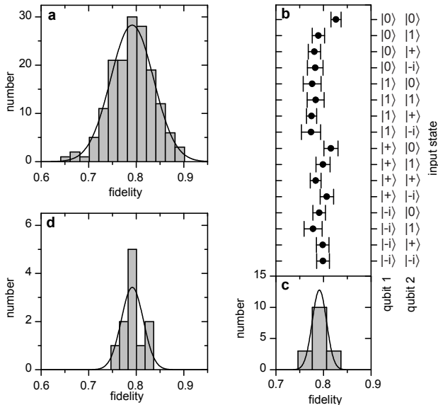
FIG. 3: Characterization of arbitrary control. a , Histogram of the output state fidelities f for 160 arbitrary unitary operations applied to one of 16 input product states. The mean output state fidelities \langle f \rangle for each input state b , plotted showing the standard error of the mean and c , binned into a histogram. d , The mean state fidelities \bar{f} for the 11 operations reconstructed using quantum process tomography. The curves are normal distributions with the same respective mean and standard deviation as the data. The narrower distributions in histograms c,d are expected because they are distributions of means.
