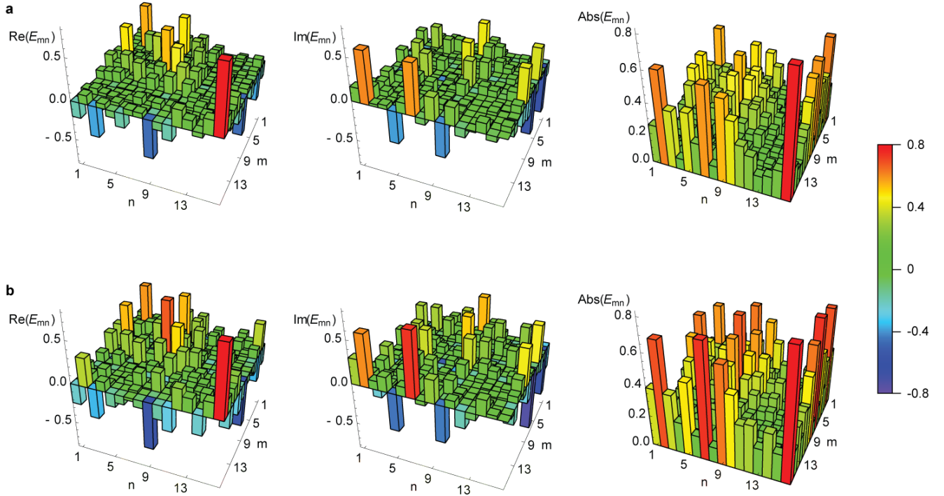
Supplementary Figure 1: Comparison of a , experimental and b , ideal process matrices of U ; the fidelities are F = 0.77 and \bar{f} = 0.82 . The process matrix E contains the maps \mathcal{E}(|i\rangle\langle j|) for all 16 elements |i\rangle\langle j| . Since each map yields a 4 \times 4 matrix \mathcal{E}_{k,l} , E is a 16 \times 16 matrix labeled by m = 4(i-1) + k , n = 4(j-1) + l . For example, the |00\rangle\langle 11| ( i = 4, j = 1 ) element of an input density matrix is mapped to \mathcal{E}(|00\rangle\langle 11|) , a 4 \times 4 block of E given by m \in [13, 16] and n \in [1, 4] .
