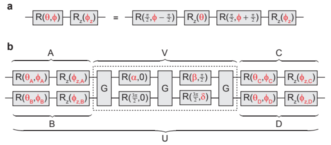
FIG. 1: Components for universal computation. Circuit diagrams for arbitrary unitary transformations on a , one and b , two qubits. The operations for each circuit are implemented from left to right with each line representing one qubit. Part a also indicates the decomposition employed for R(\theta, \phi) . The dashed box in part b contains the three degrees of freedom \alpha, \beta, \delta that determine the two-qubit operation’s local equivalence class. The brackets highlight the decomposition of the two-qubit operation U as described in the text: U = (C \otimes D) \cdot V \cdot (A \otimes B) .
